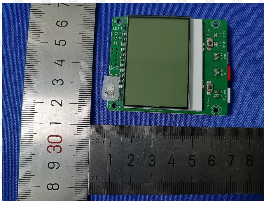
Photo 13: PCB view
